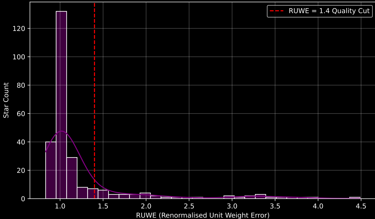
GALAH DR4 Field [1223] RUWE Distribution (n= 255)
