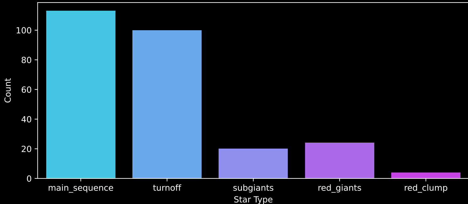
GALAH DR4 Field: [1223] Count plot of Star Type
