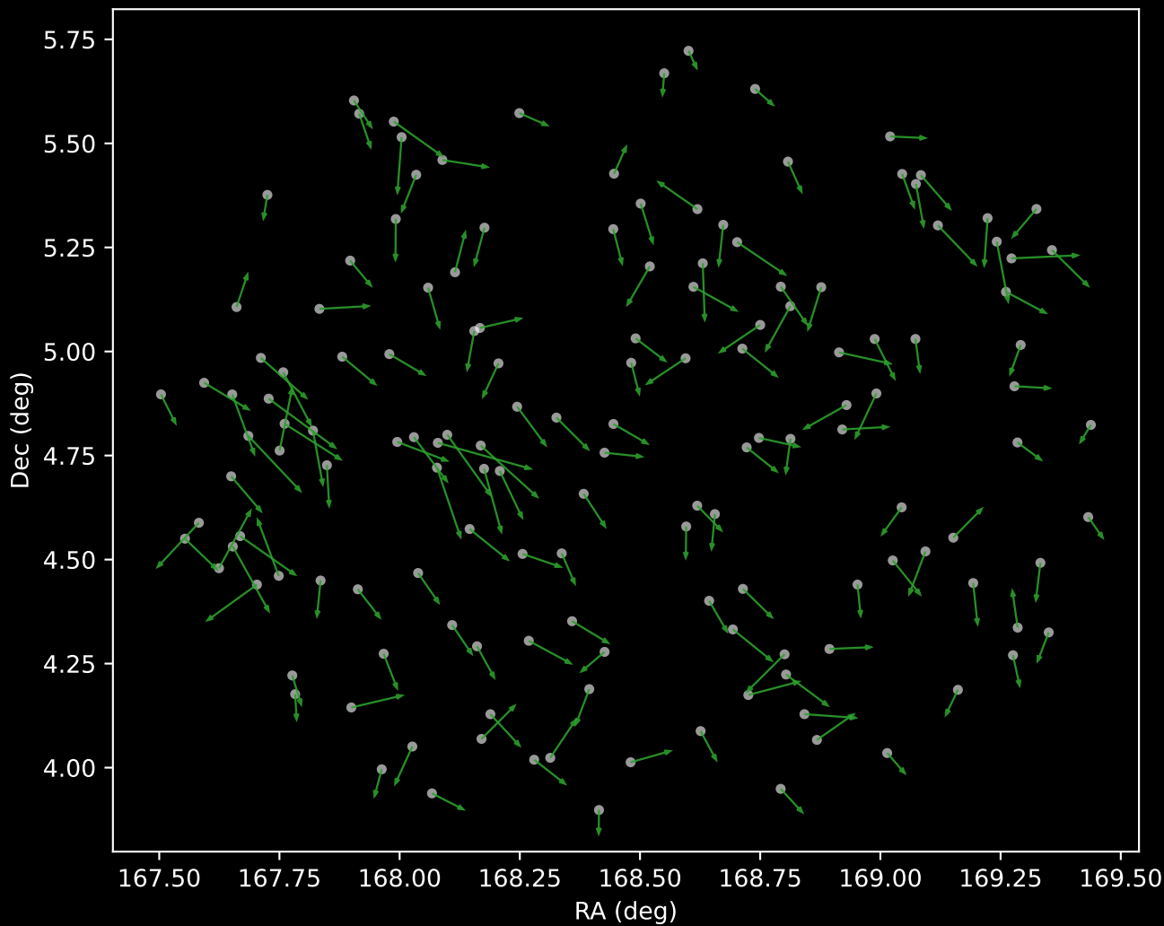
GALAH DR4 Cluster 4 Proper Motion Vectors (n=149)
